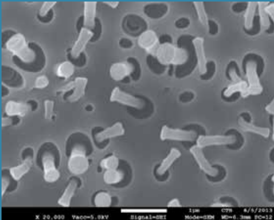
Microfibrils cross section - SEM image
